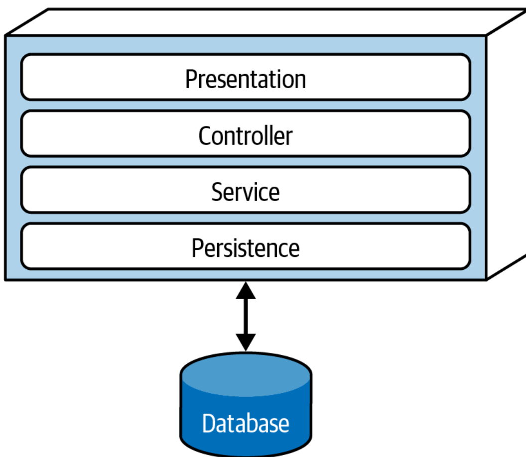
Figure 6-4. Layered architecture
